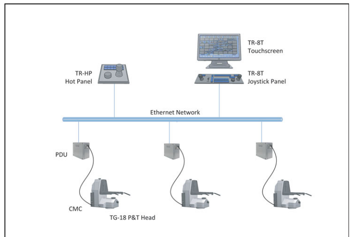
3 Camera System with TR-T Controller and TR-HP Hot Panel
