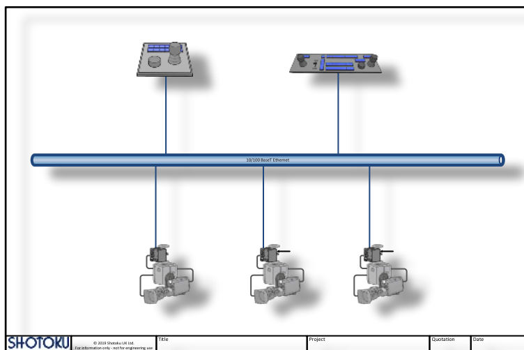
3 Camera System with TR-B Panel and TR-HP Hot Panel
